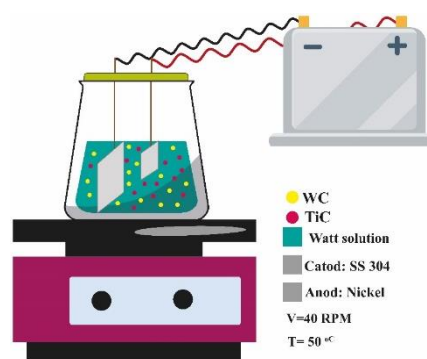
Fig. 1. Schematic of the Watts solution used in the coating process
